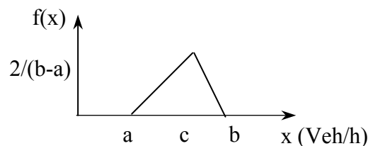
Figure 2. Triang(a,b,c) Density Function
