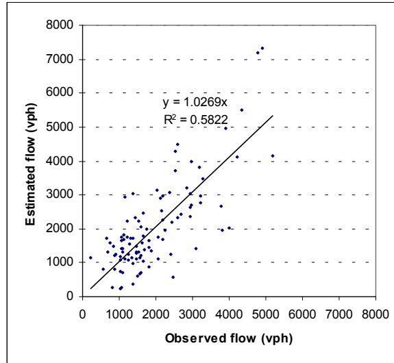
Figure 3. Correlation Between Observed And Those Estimated Link Flows
