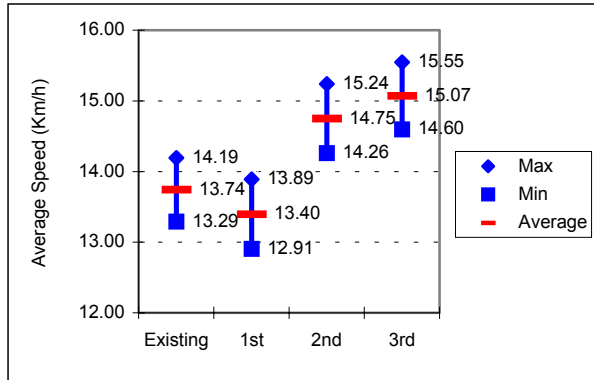
Figure 8a. Interval of Total Veh-Km for each scenario
